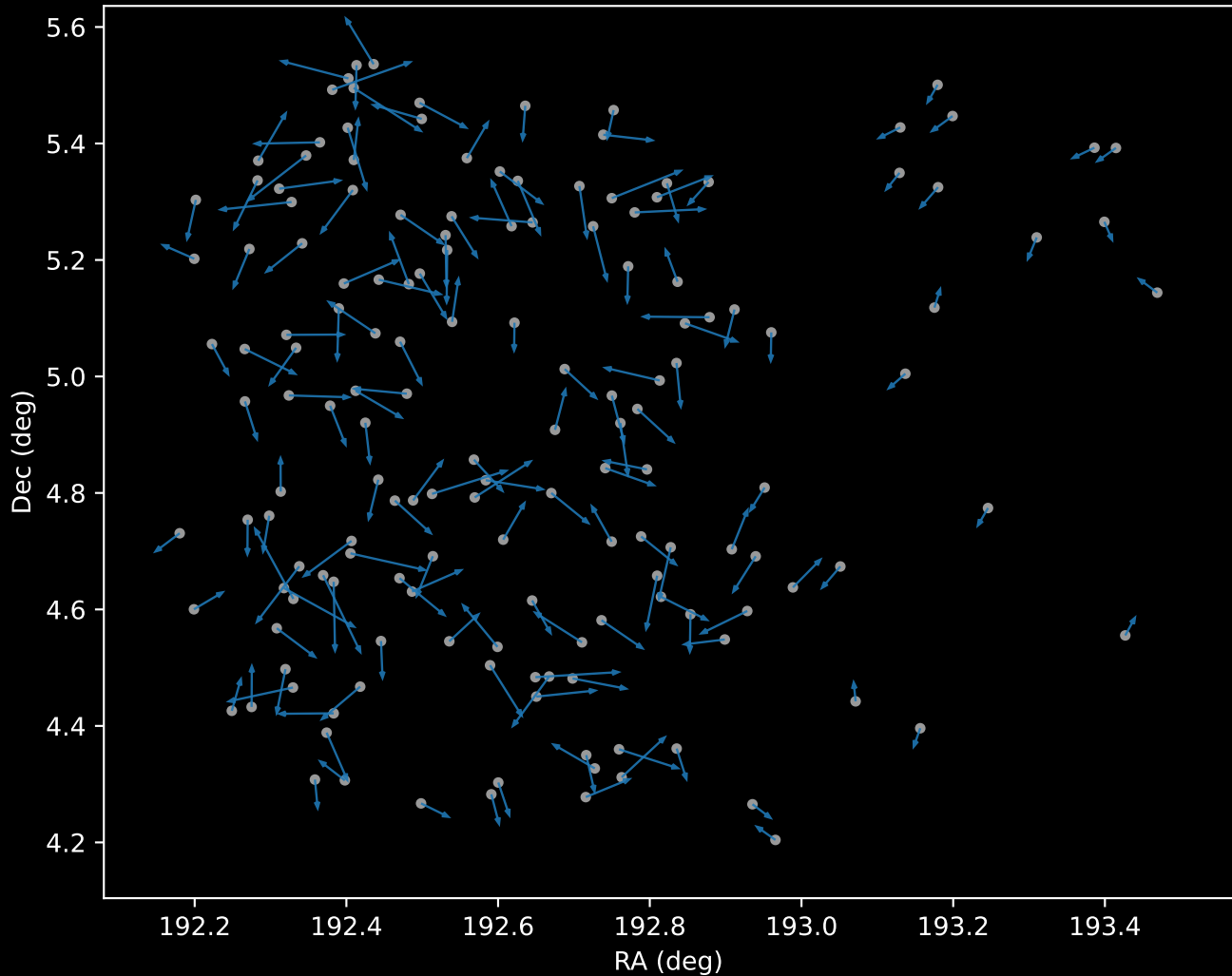
APOGEE DR17 Cluster 0 Proper Motion Vectors (n=158)
