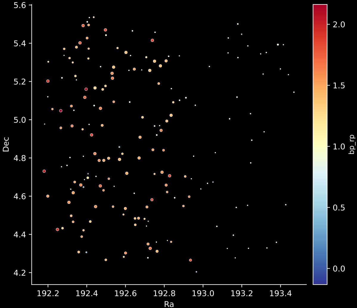
APOGEE DR17 Field: [203-06-C] Stars: 187
