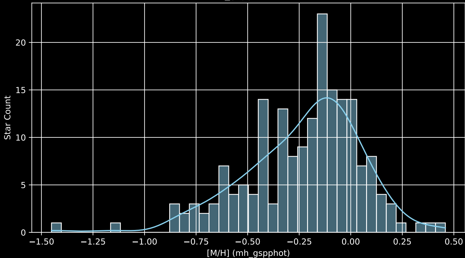
APOGEE DR17 Field: [203-06-C [M/H] (mh_gspphot) (n= 186)
