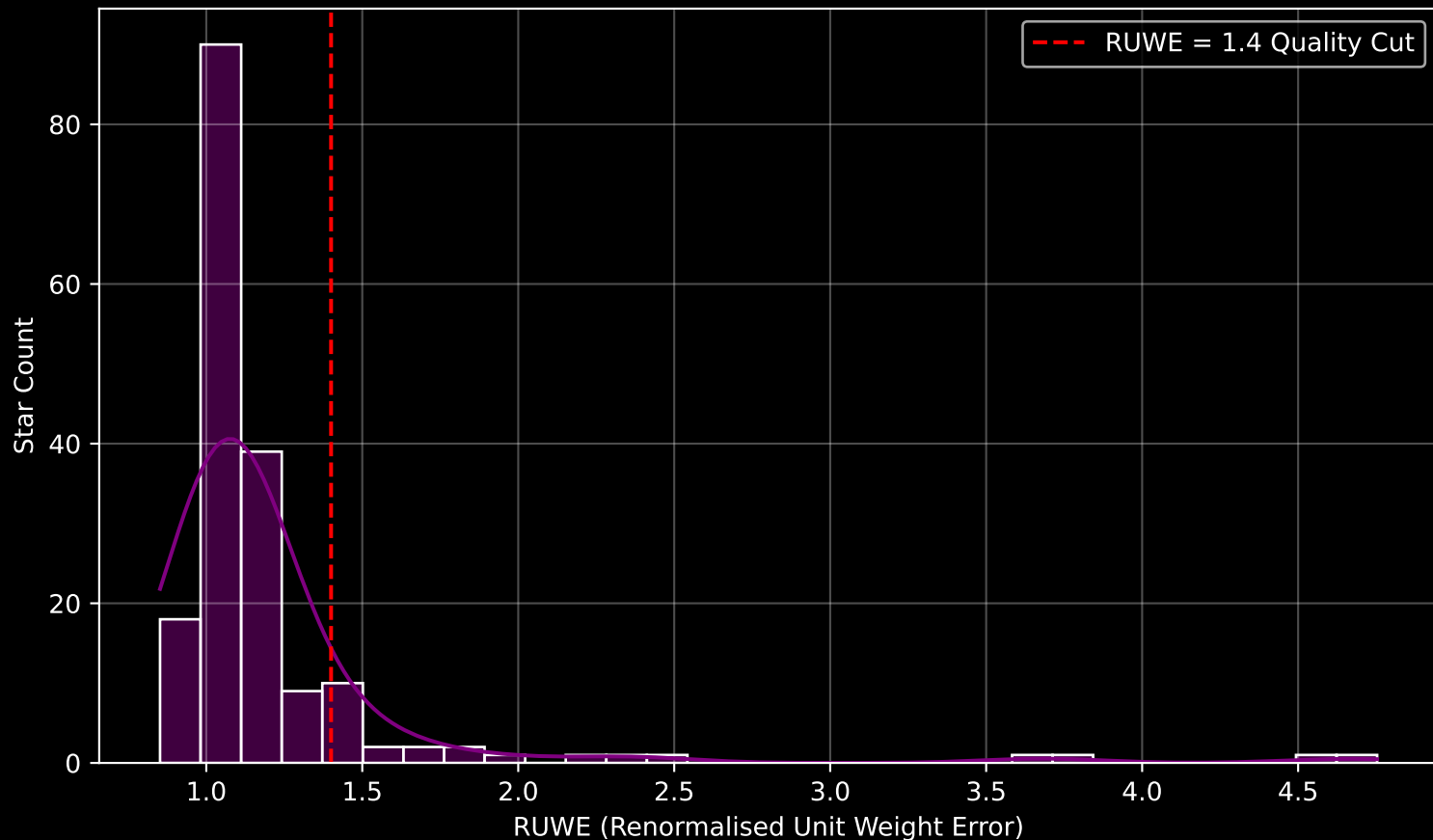
GAPOGEE DR17 Field [203-06-C] RUWE Distribution (n= 180)
