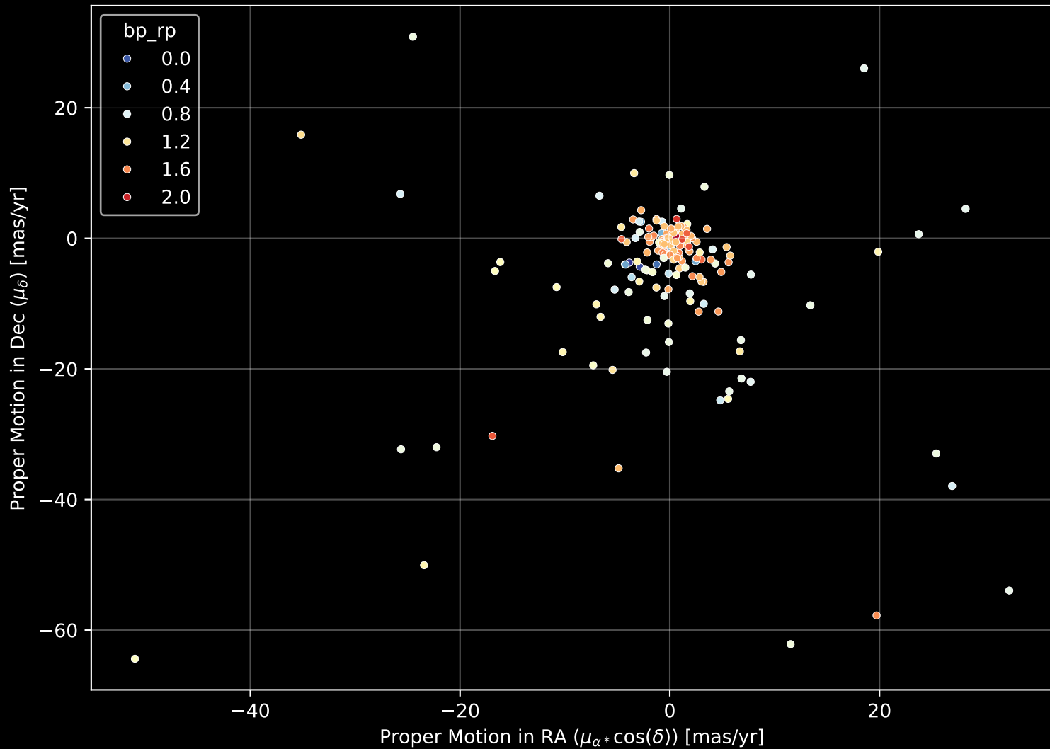
APOGEE DR17 Field: [203-06-C] Proper Motion Diagram (n= 187)
