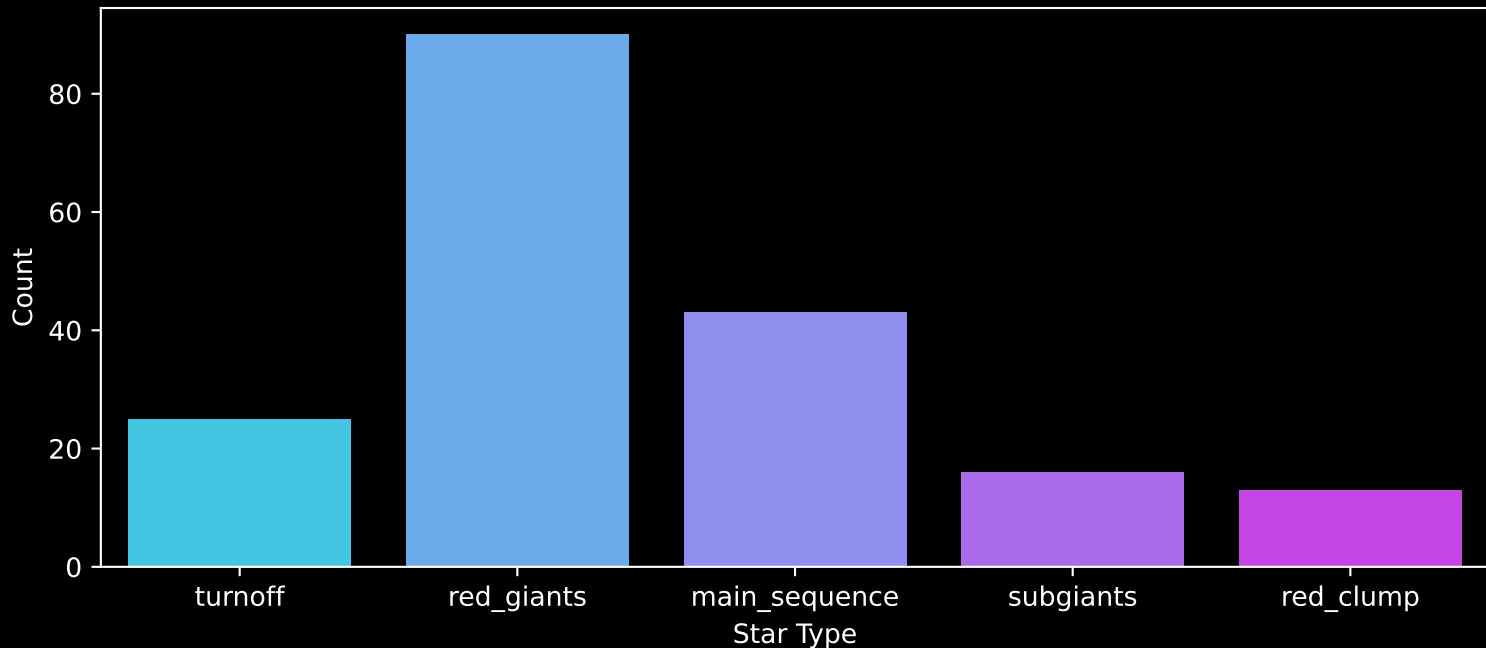
APOGEE DR17 Field: [203-06-C] Count plot of Star Type
