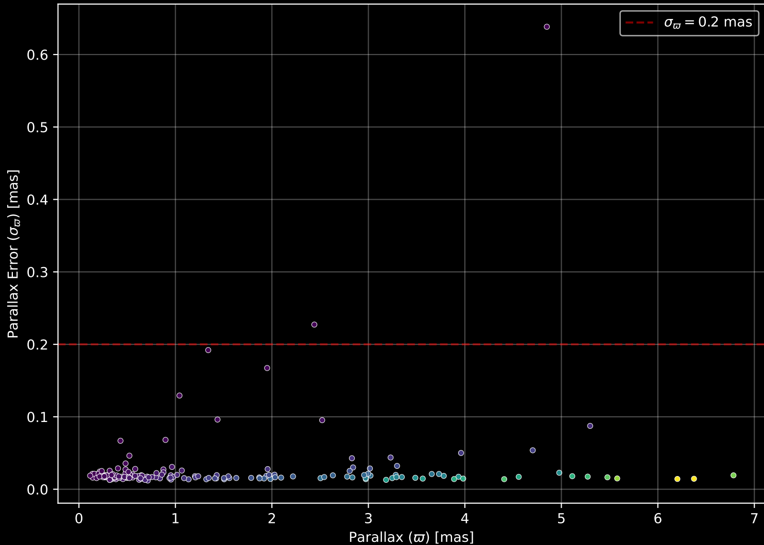
APOGEE DR17 Field: [203-06-C] Parallax Quality (n= 187)
