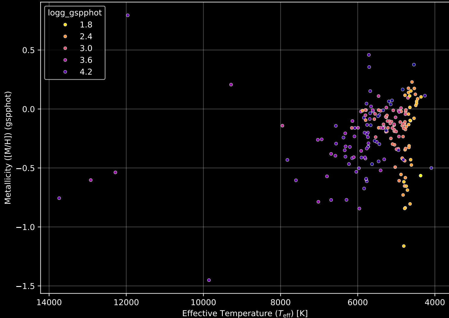
APOGEE DR17 Field: [203-06-C] Stellar Population Parameters (n= 187)
